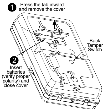
Figure 4: Battery Replacement
