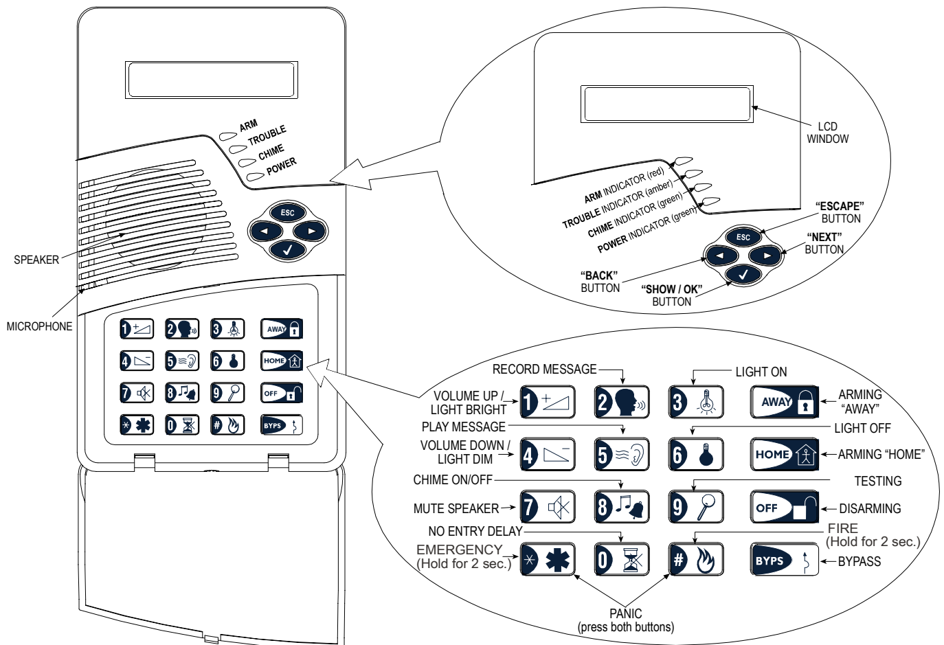
Figure 1: External View
